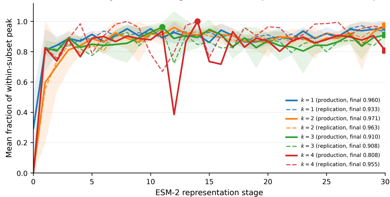
A Order-level dynamics through ESM-2 (solid=production, dashed=replication)
