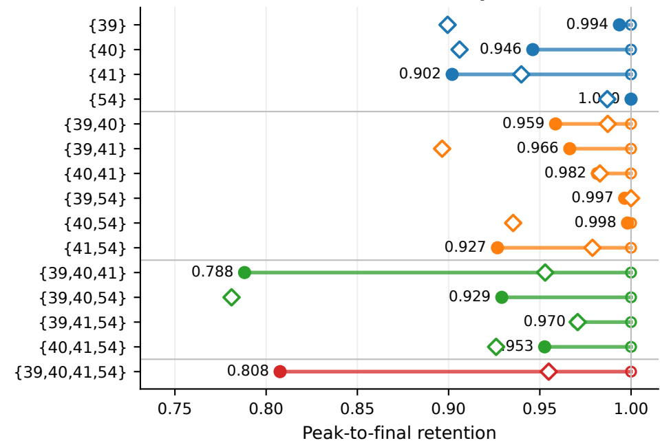
C What survives to the final representation? (● production, ◇ replication)
